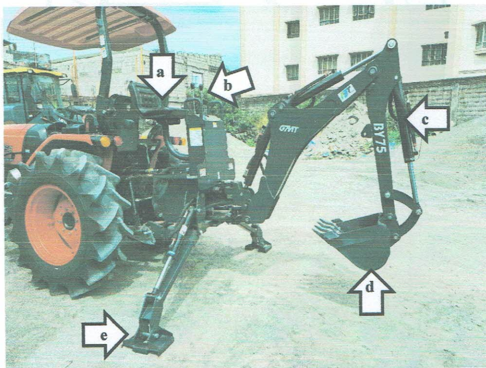
Figure 1. Parts of the GMT BY75P Backhoe powered by 40.5 kW TYM 5825R Four-Wheel Tractor include the following: (a) Operator's seat, (b) Controls, (c) Backhoe arm, (d) Bucket, and (e) Stabilizer.
