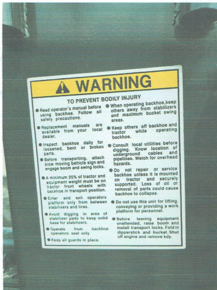
Figure 5. Warning sticker of the GMT BY75P Backhoe.
